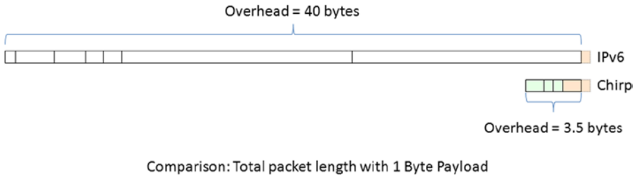
Figure 2-5. Comparison of TCP/IP packet and chirp packet overheads for a 1-byte payload from a simple sensor
